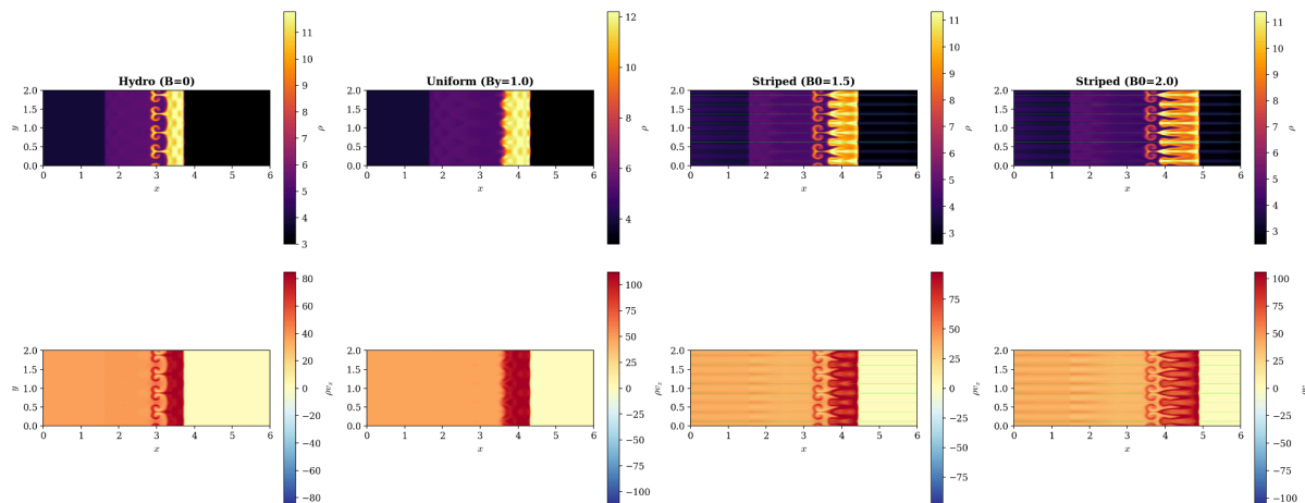
Magnetic Nozzle: Splash vs Focused Jets (top: density, bottom: x-momentum)
